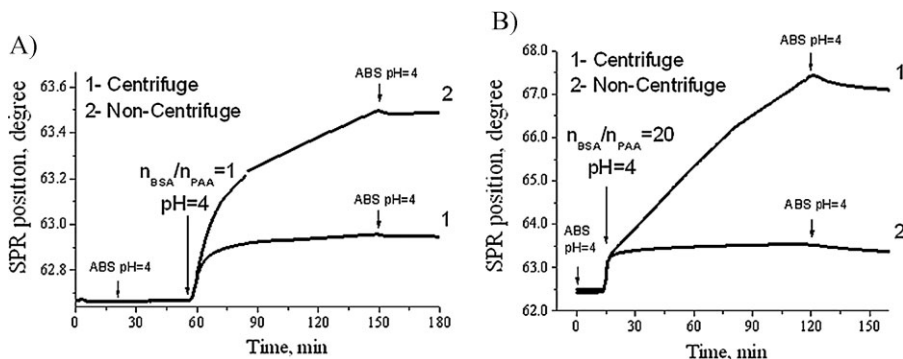
Figure 1. Temporary dependence of SPR angle position on sedimentation of PCs, n_{\text{BSA}}/n_{\text{PAA}} = 1.0 (A) and n_{\text{BSA}}/n_{\text{PAA}} = 20 (B) at pH 4.0; 25 °C.
