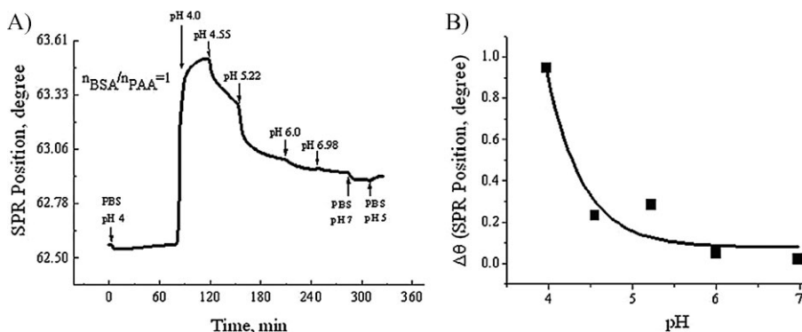
Figure 2. (A) Kinetic dependence of SPR angular position, that reflects conformational changes in structures of PAA-BSA mixture at the ratio of n_{\text{BSA}}/n_{\text{PAA}} = 1.0 when the overlayer pH was changed from acidic to basic (pH 4.0 → pH 6.98). The horizontal part of graph- gold surface is without PAA/BSA layer. (B) Maximum of SPR responses depending on the wide range of pHs.
